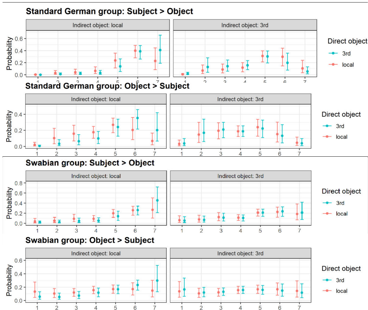
Figure 1: Standard German (top) and Swabian (bottom) speakers' acceptability ratings for the sentences of the experiment. Points indicate posterior mean estimates for the probability that the ratings fall into the seven rating categories and error bars indicate 95% credible intervals.
